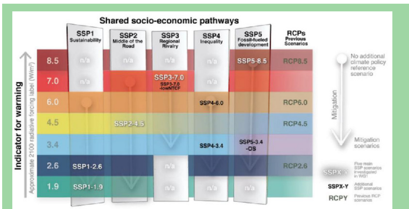
Figure 2 - The SSP scenarios used in the IPCC 6AR, their indicative temperature evolution and radiative forcing categorization, and the five Shared Socio-economic Pathways (SSP) upon which they are built.
